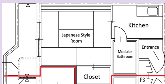
Layout of a room (21.33m²)
